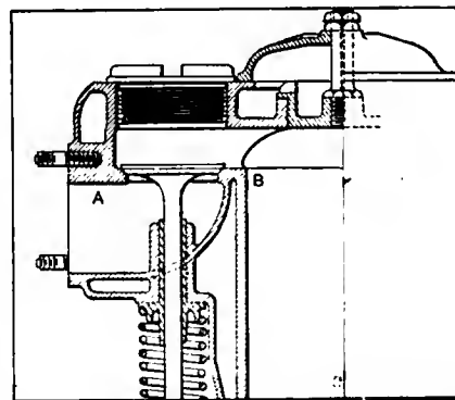
Fig. 3—Section through the cylinder of a motor in which the water-cooling area is bad
